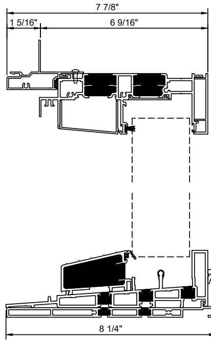
Standard 6/9 Sill Operable Side
