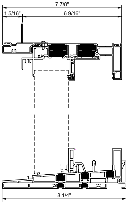
Standard 6/9 Sill Fixed Side
