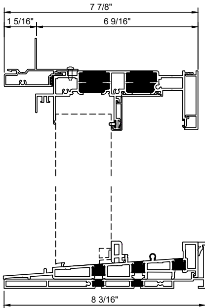
Low Profile 6/9 Sill Fixed Side
