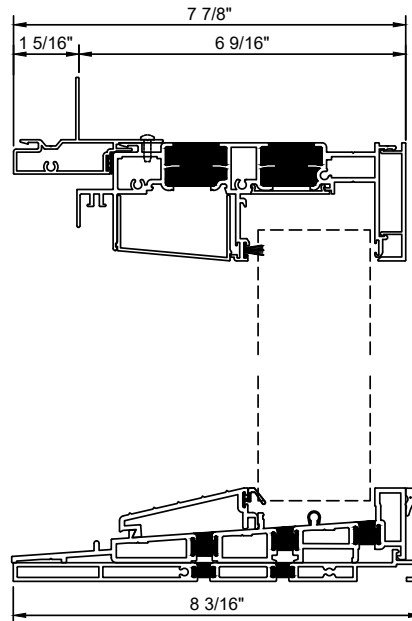
Low Profile 6/9 Sill Operable Side
